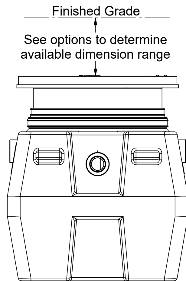
END VIEW
