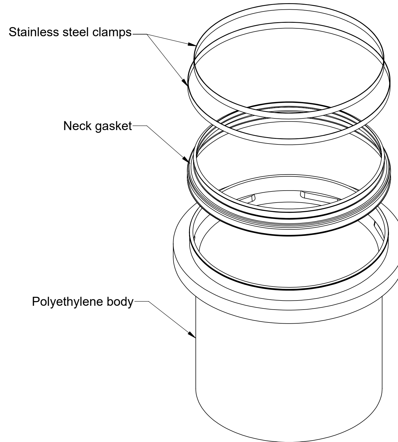
EXPLODED VIEW
