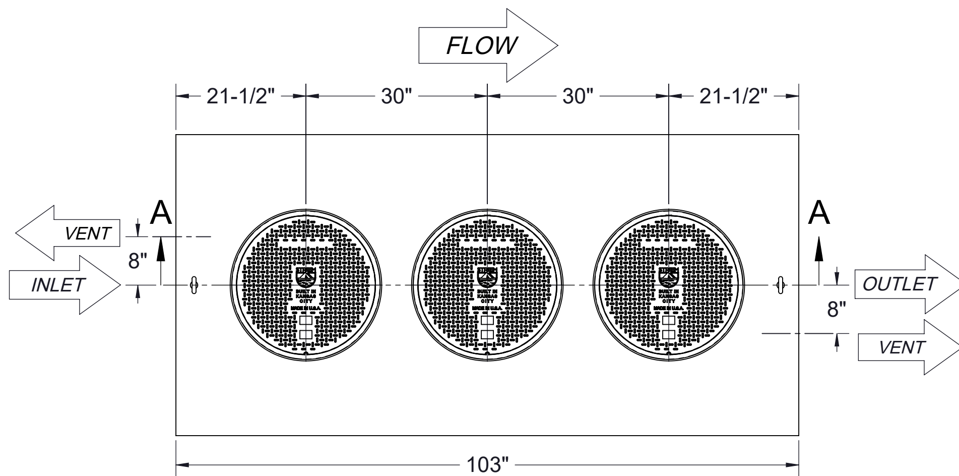
TOP VIEW
