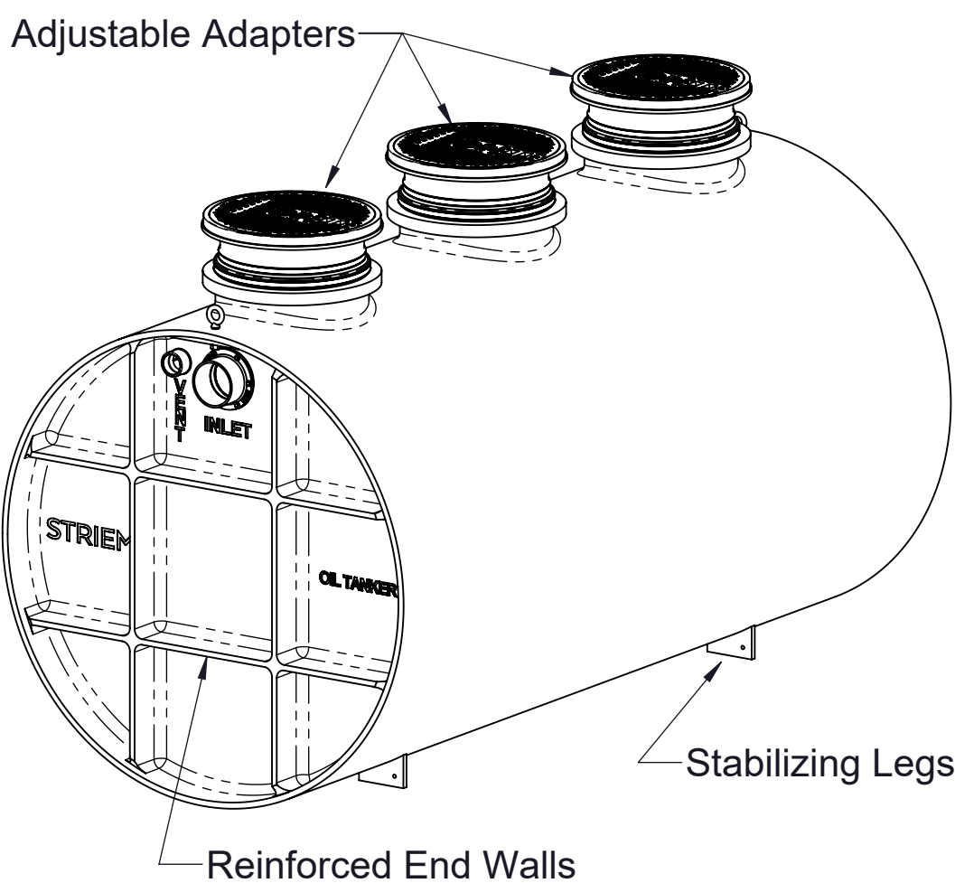
ISOMETRIC VIEW
