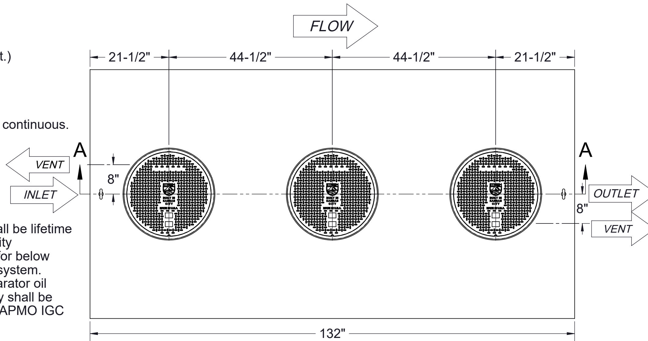
TOP VIEW
