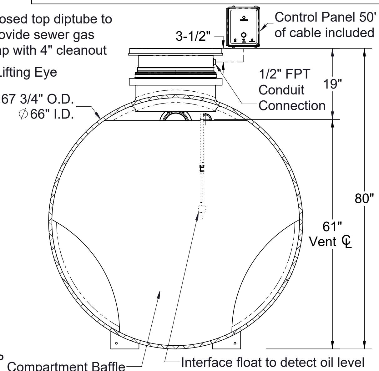
SECTION B-B
