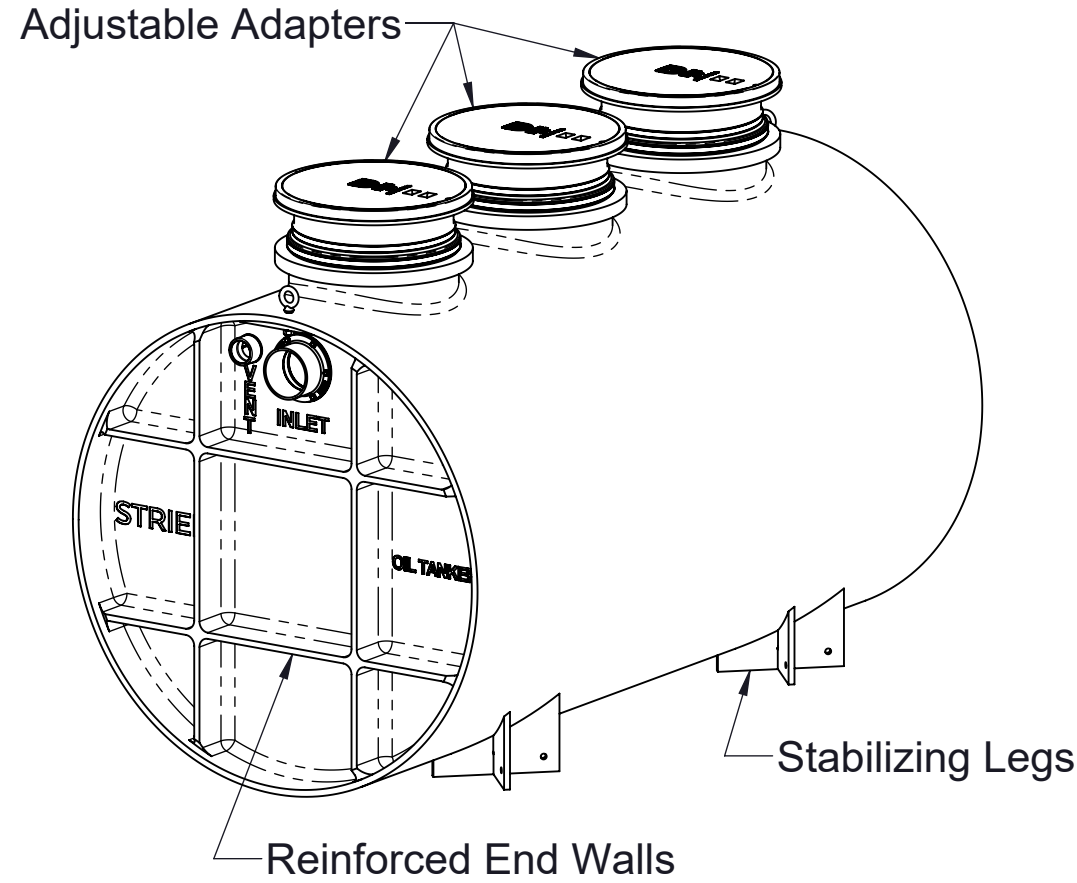
ISOMETRIC VIEW
