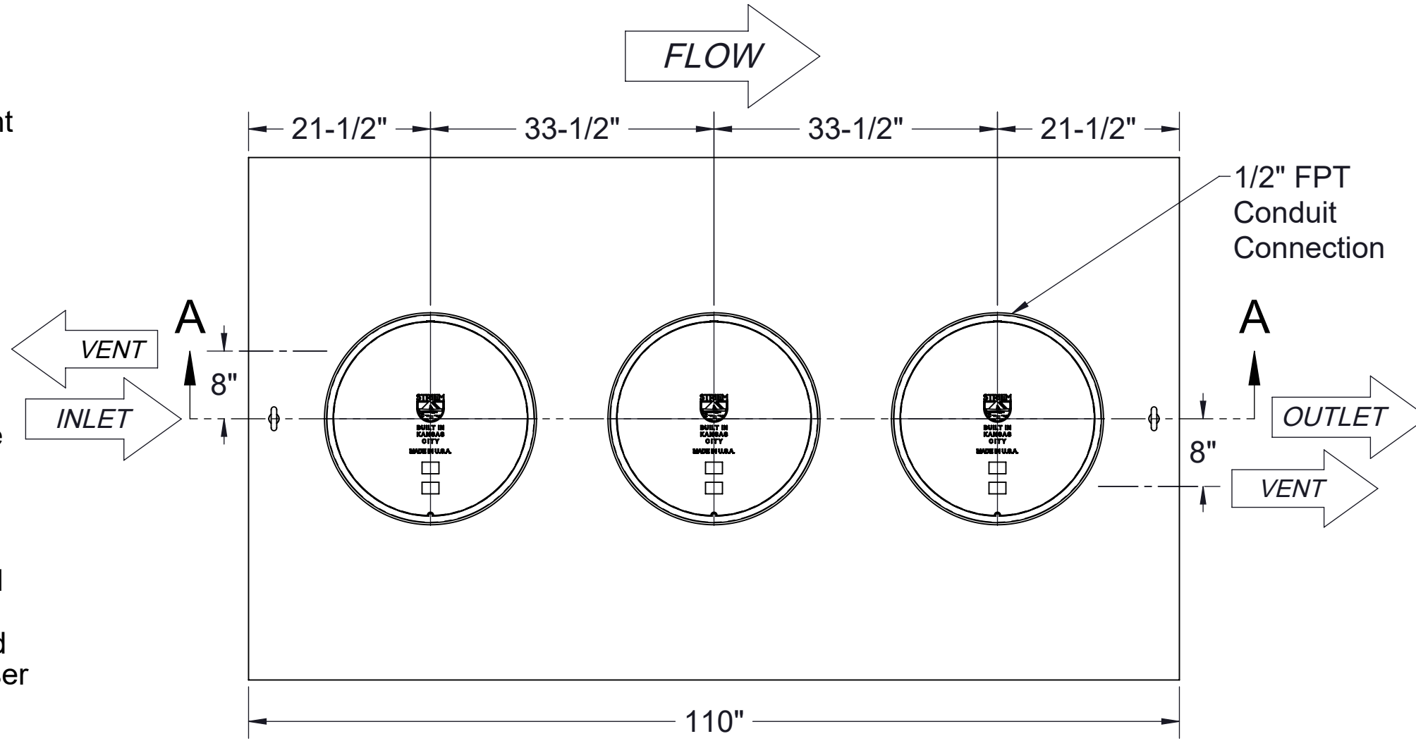
TOP VIEW
