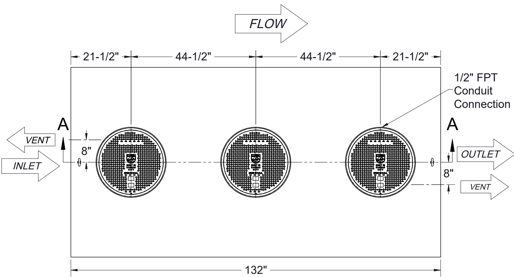
TOP VIEW
