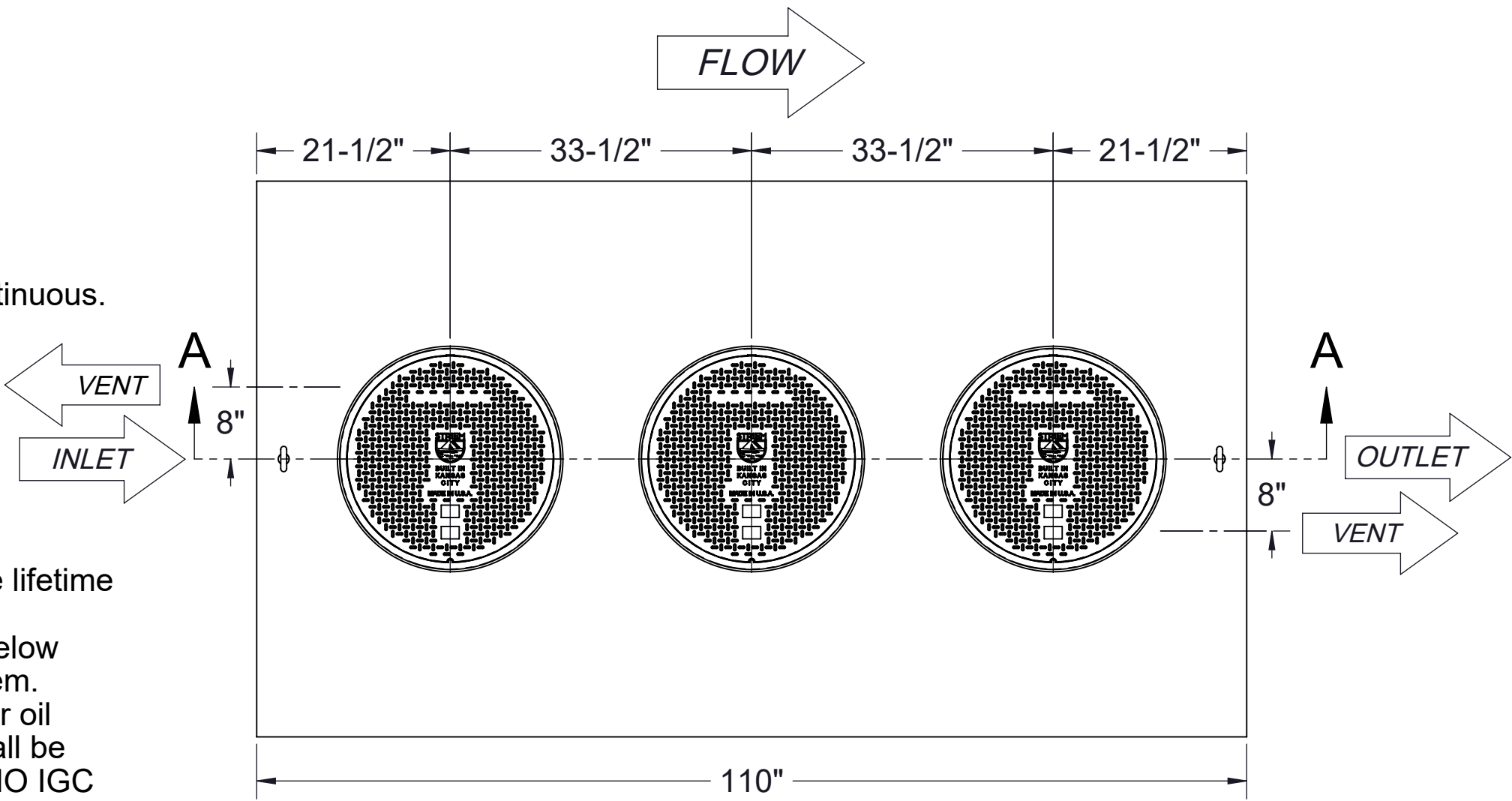
TOP VIEW
