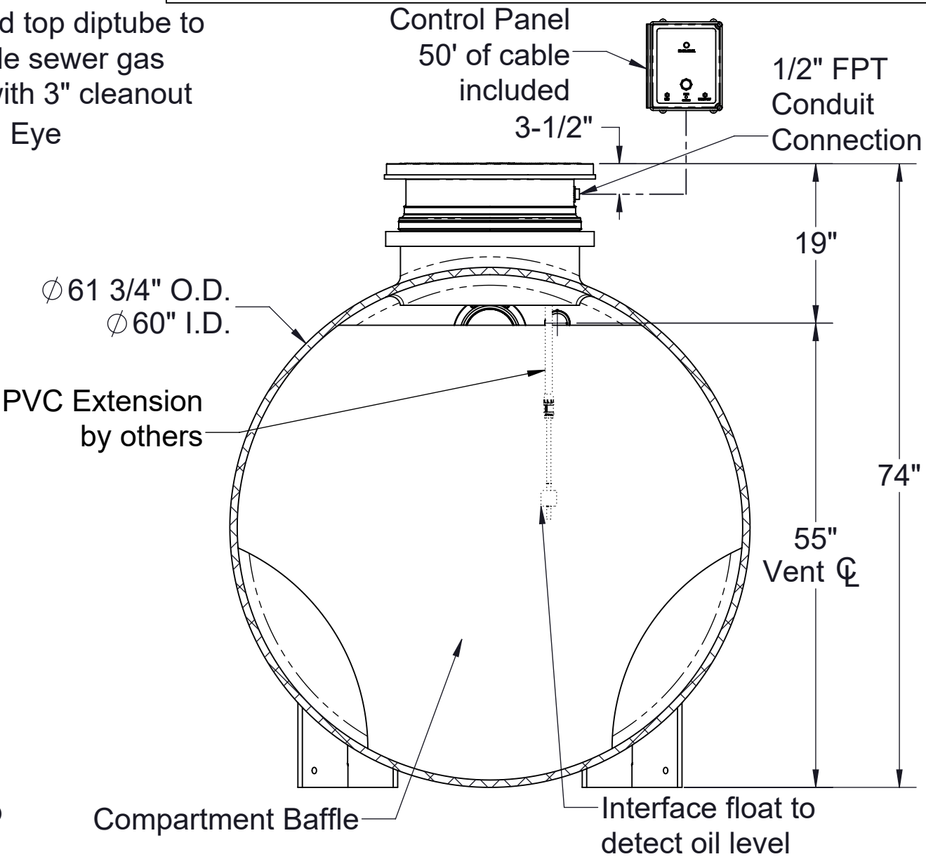
SECTION B-B
