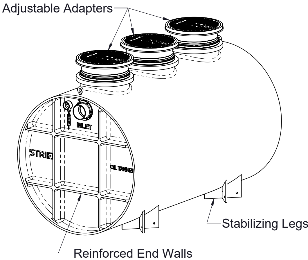
ISOMETRIC VIEW
