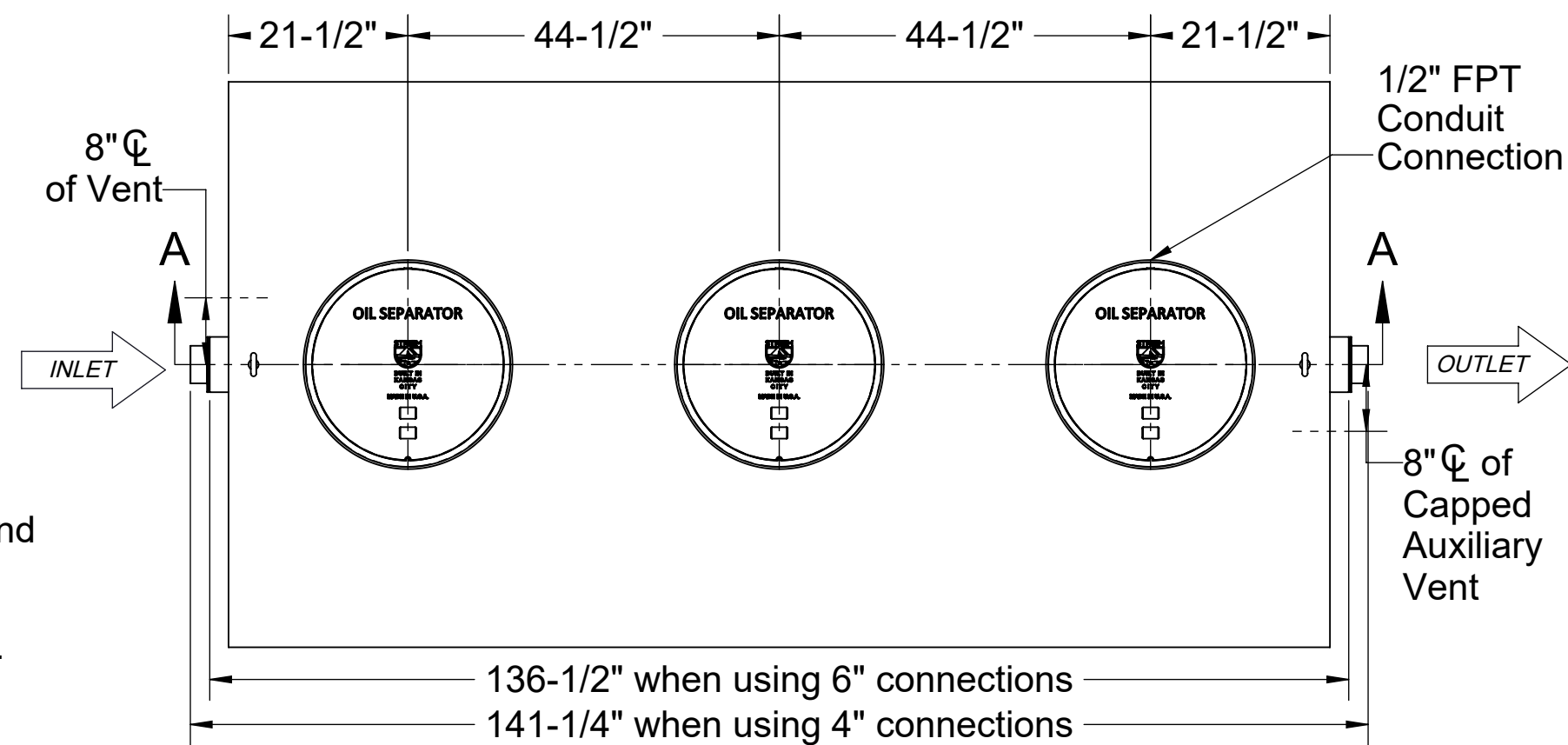
TOP VIEW
