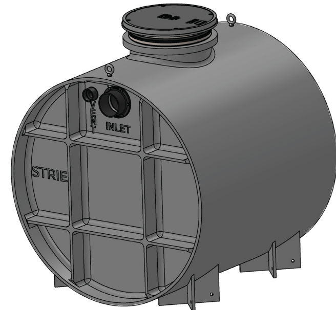
LB-500 LB SERIES 500 GALLON NEUTRALIZATION TANK
