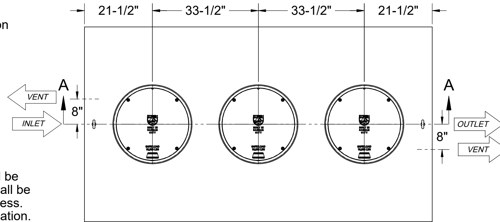
TOP VIEW
