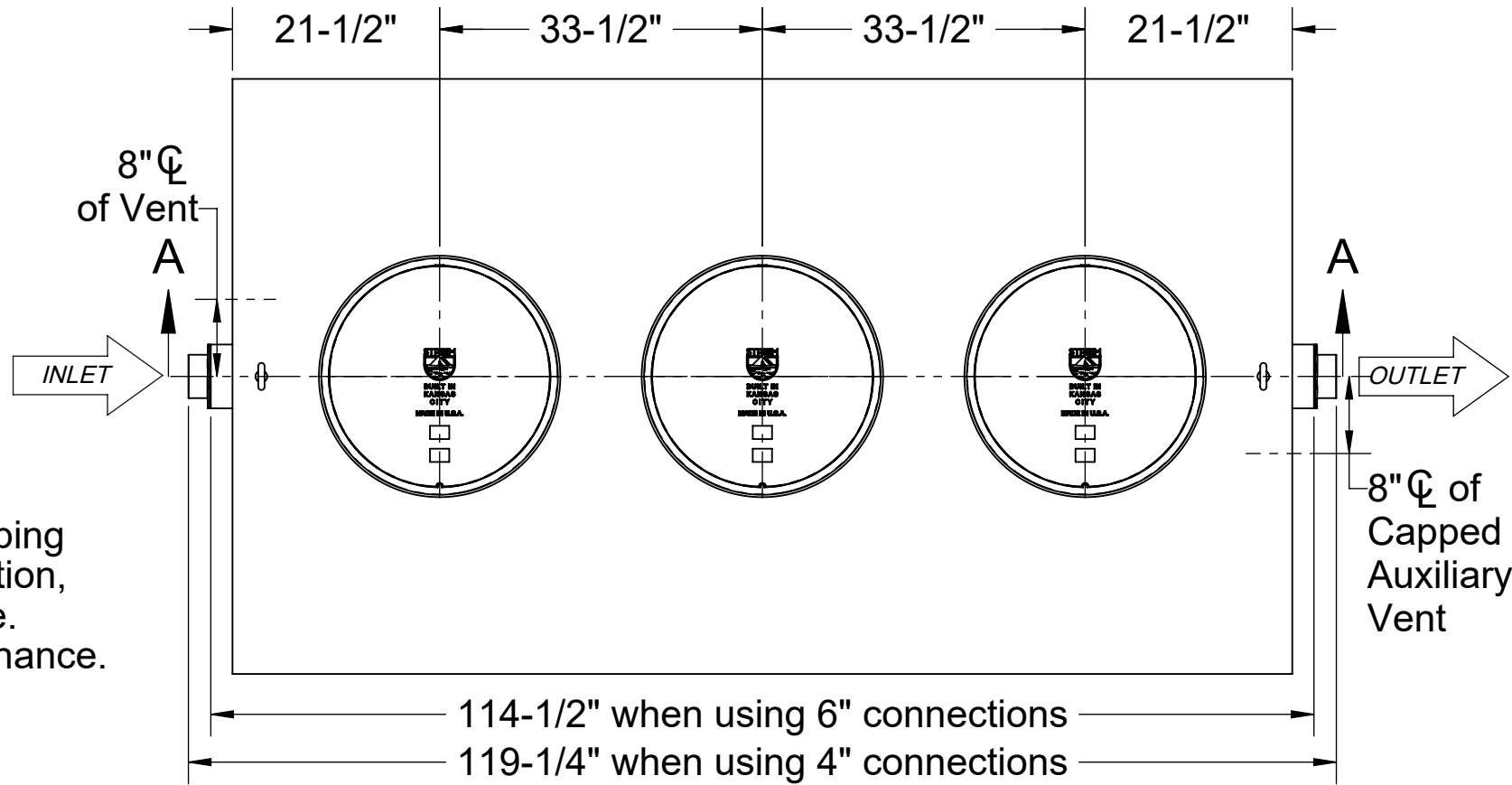
TOP VIEW
