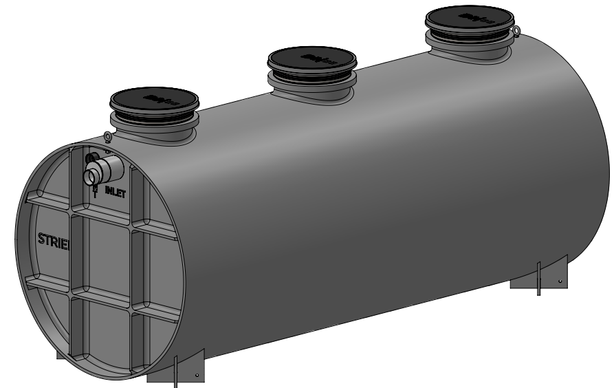
FLI-1500 FLAMMABLE LIQUID INTERCEPTOR 1,500 GAL
