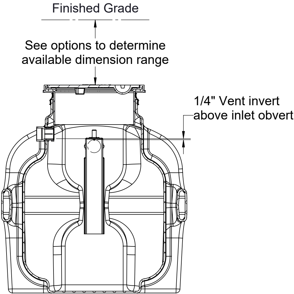
SECTION B-B
