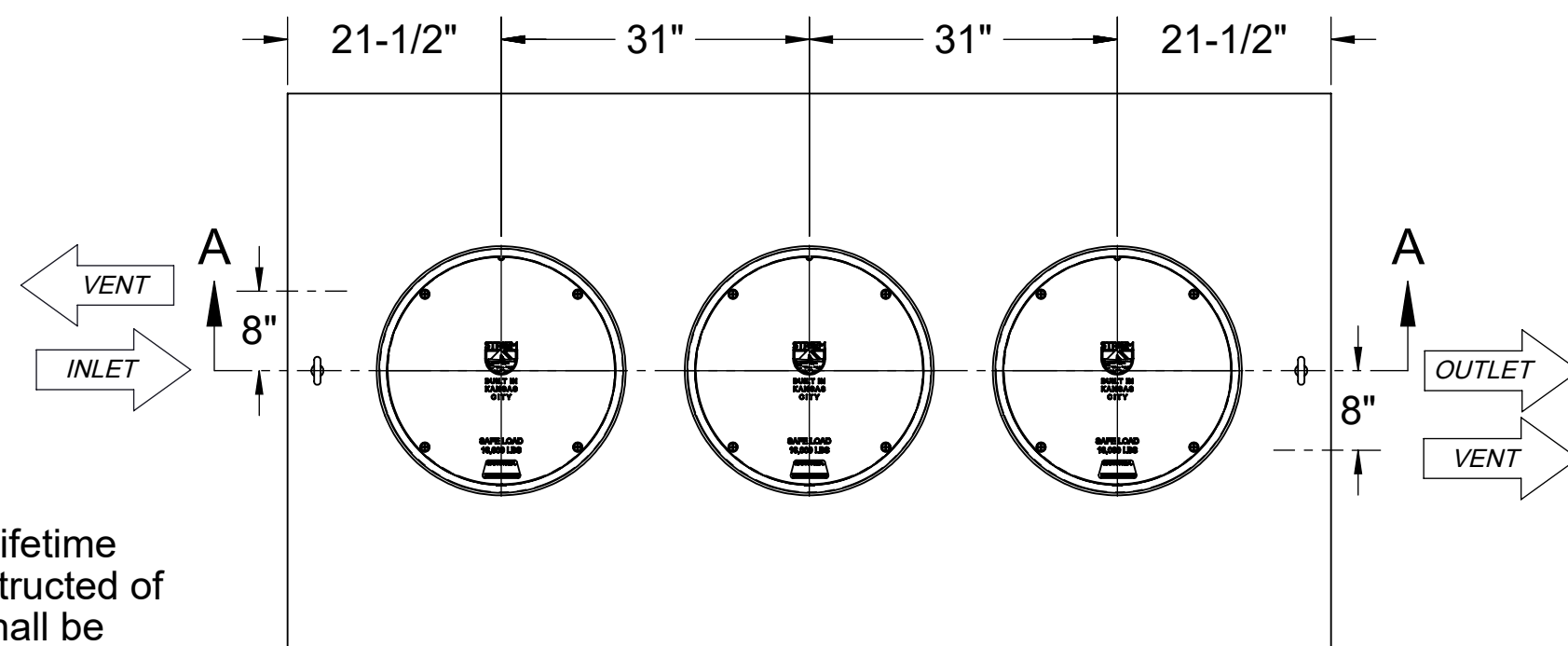
TOP VIEW
