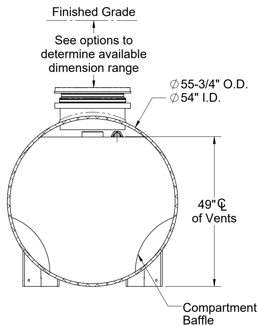
SECTION B-B
