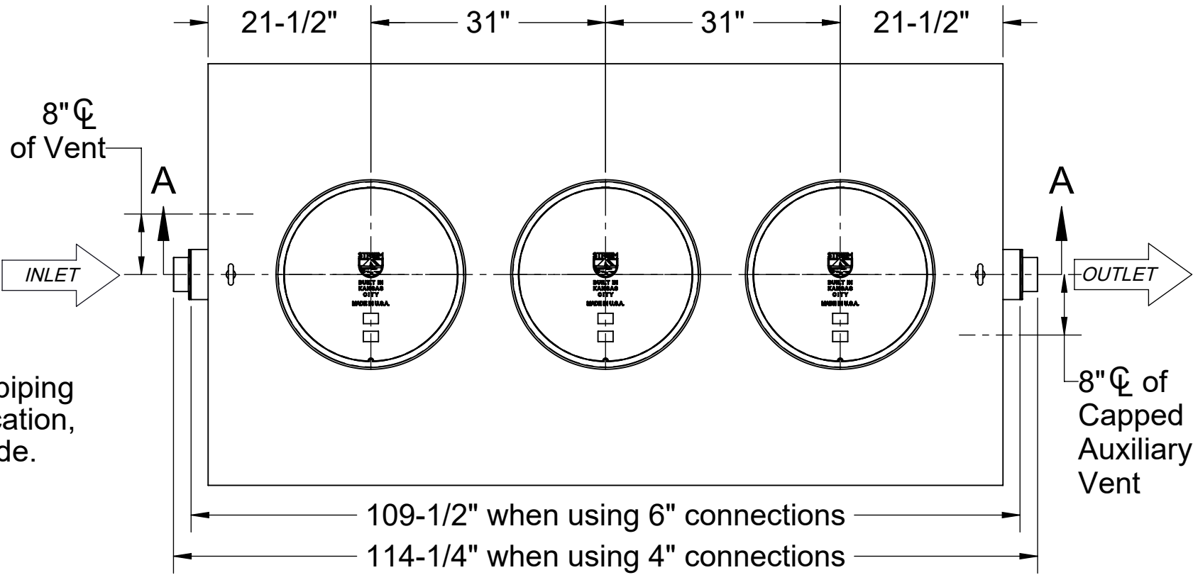
TOP VIEW
