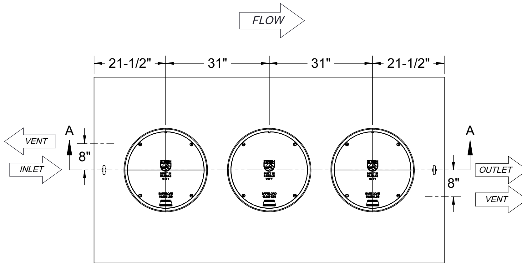
TOP VIEW
