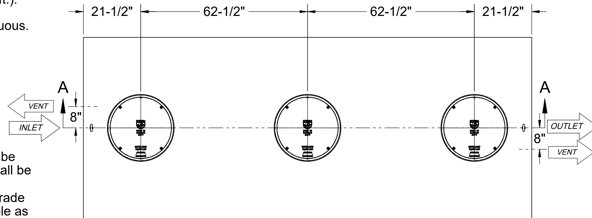
TOP VIEW
