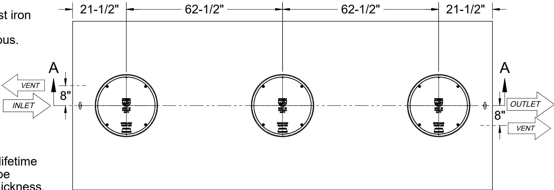
TOP VIEW
