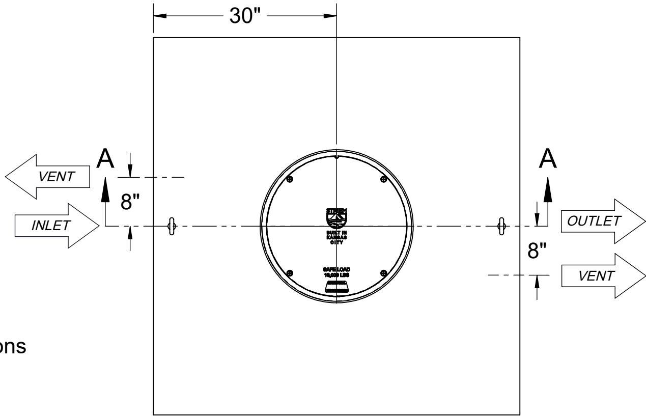
TOP VIEW
