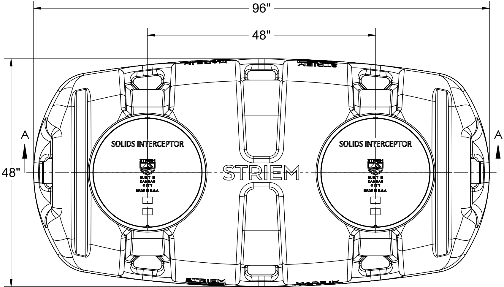
TOP VIEW
