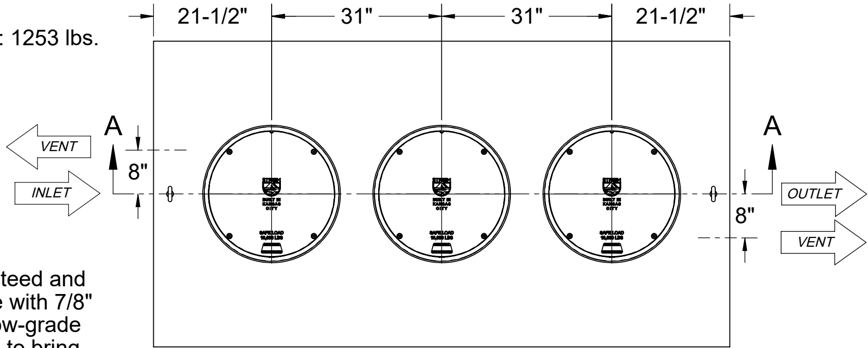
TOP VIEW
