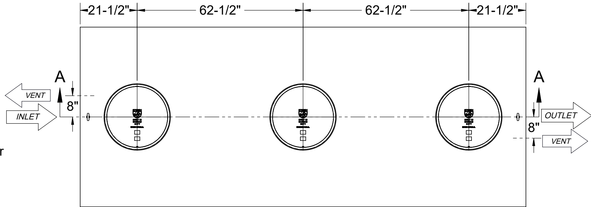
TOP VIEW
