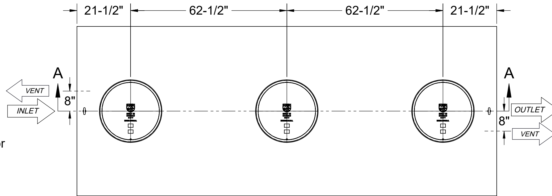
TOP VIEW
