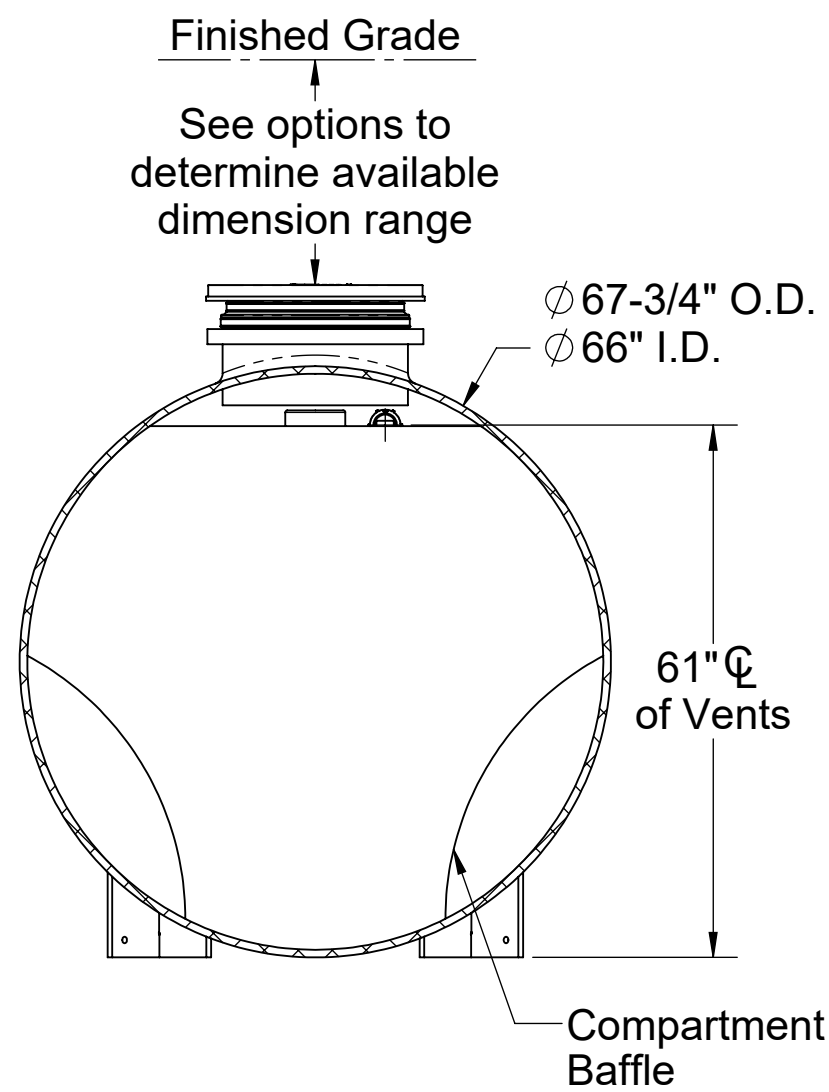
SECTION B-B
