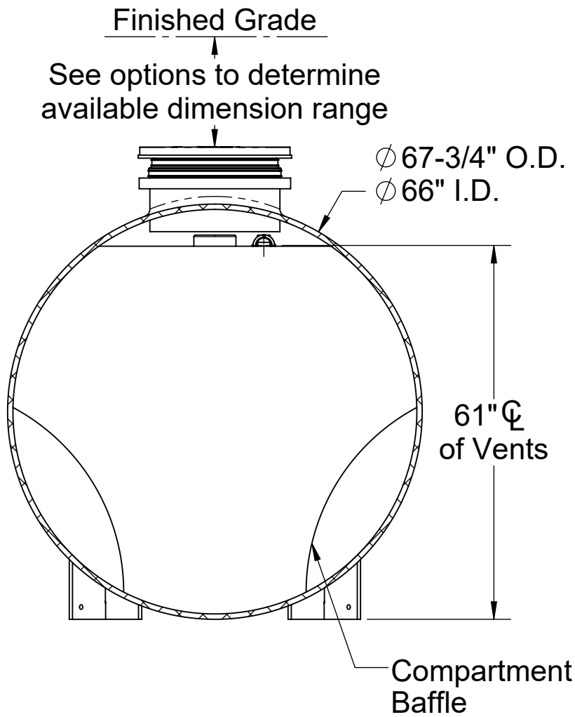
SECTION B-B
