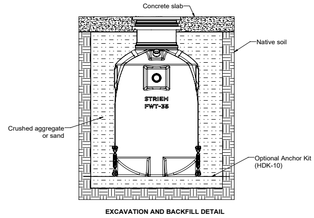
EXCAVATION AND BACKFILL DETAIL
