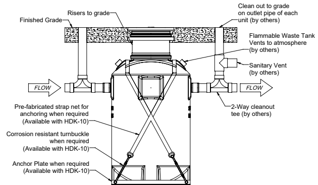
EXCAVATION AND BACKFILL DETAIL
