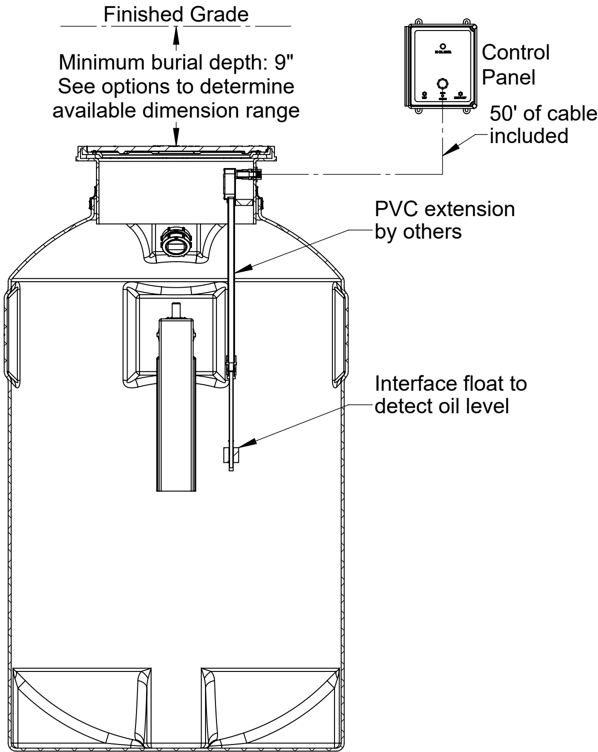
SECTION B-B
