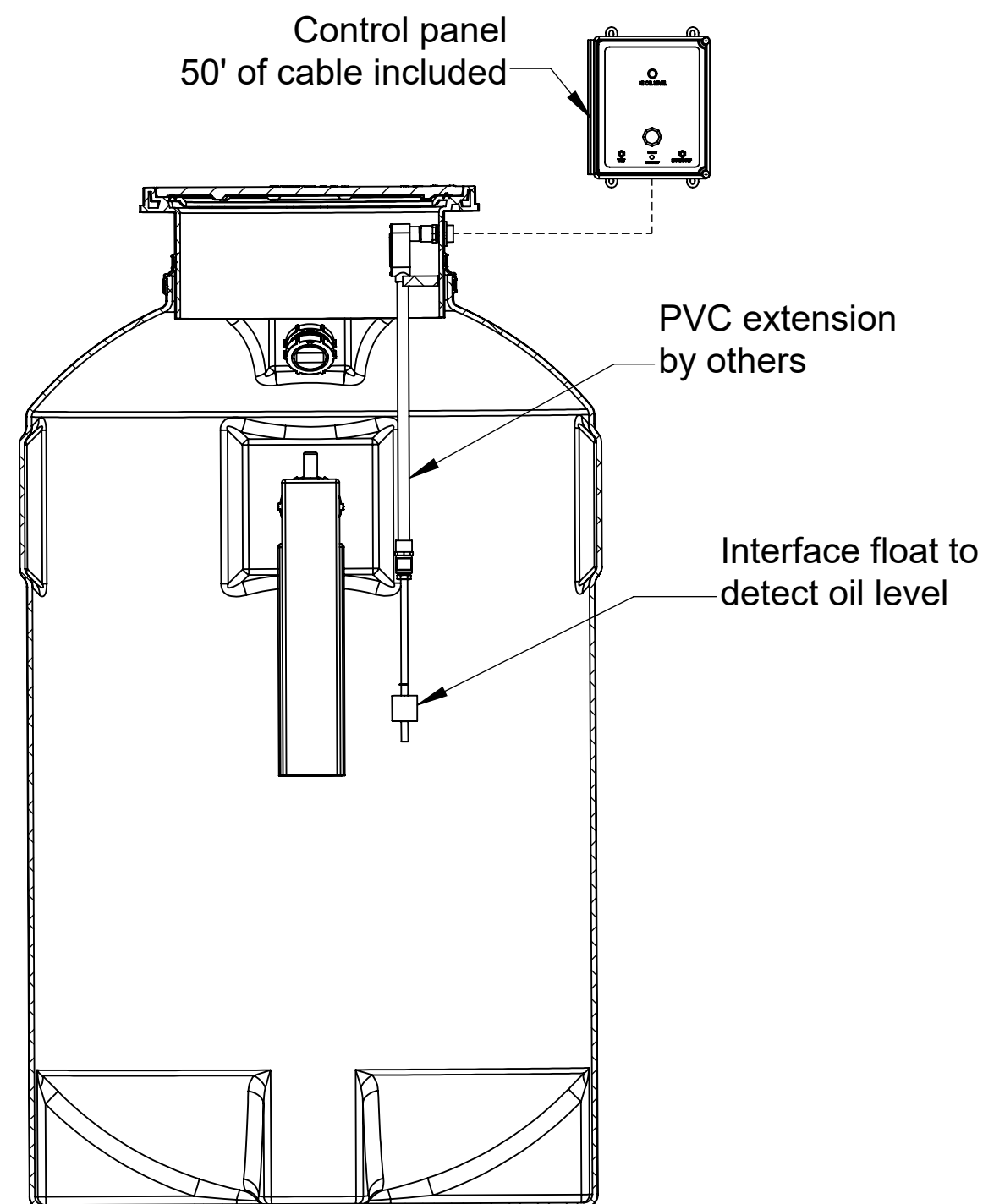
SECTION B-B
