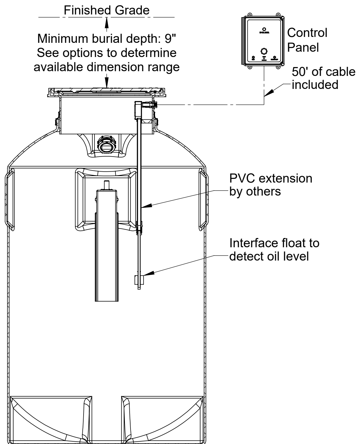
SECTION B-B
