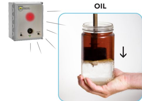
Float is in "DOWN/CLOSED" position in oil, sounding an alarm
