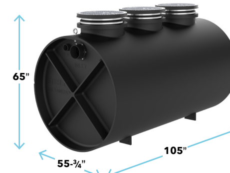
LB-750 OPTIONS 24" CPRK HDK LS CC-1 CONNECTIONS: 4", 6", 8" LIMESTONE LOAD: 9,800 LBS. # OF LAB SINKS: 215 COVER: TRAFFIC-RATED
