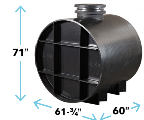
CB-500-S OPTIONS → H-20 24" CPRK HDK
