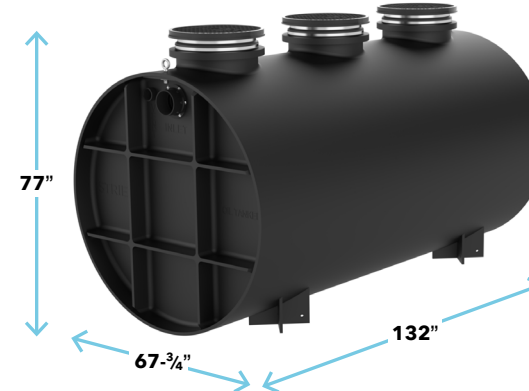
LB-1500 OPTIONS 24" CPRK HDK LS CC-1 CONNECTIONS: 4", 6", 8" LIMESTONE LOAD: 19,500 LBS. # OF LAB SINKS: 375 COVER: TRAFFIC-RATED
