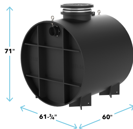
LB-500 OPTIONS 24" CPRK HDK LS CC-1 CONNECTIONS: 4", 6", 8" LIMESTONE LOAD: 6,500 LBS. # OF LAB SINKS: 150 COVER: TRAFFIC-RATED
