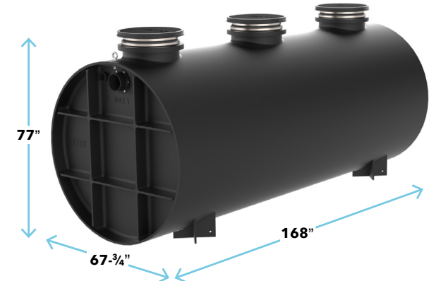
LB-2000 OPTIONS 24" CPRK HDK LS CC-1 CONNECTIONS: 4", 6", 8" LIMESTONE LOAD: 25,500 LBS. # OF LAB SINKS: 500 COVER: TRAFFIC-RATED
