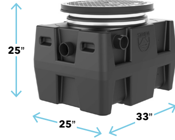
LB-35 OPTIONS 24" LS CC-1 CONNECTIONS: 2", 3", 4" LIMESTONE LOAD: 450 LBS. # OF LAB SINKS: 9 COVER: PEDESTRIAN-RATED
