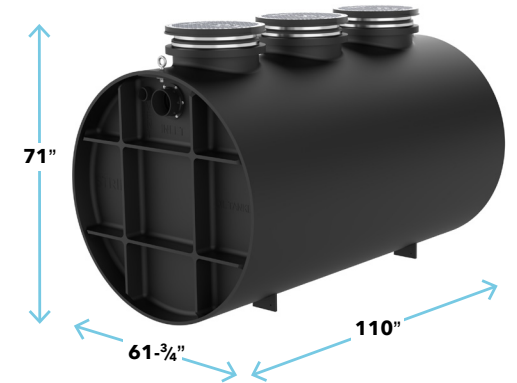
LB-1000 OPTIONS 24" CPRK HDK LS CC-1 CONNECTIONS: 4", 6", 8" LIMESTONE LOAD: 13,000 LBS. # OF LAB SINKS: 260 COVER: TRAFFIC-RATED
