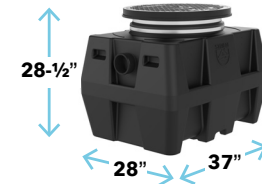
CB-50-S OPTIONS → H-20 24" HDK
