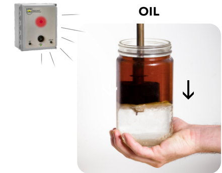
Float is in "DOWN/CLOSED" position in oil, sounding an alarm
