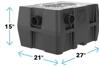
LB-25 OPTIONS 16" LS CC-1 CONNECTIONS: 2", 3" LIMESTONE LOAD: 300 LBS. # OF LAB SINKS: 6 COVER: PEDESTRIAN-RATED
