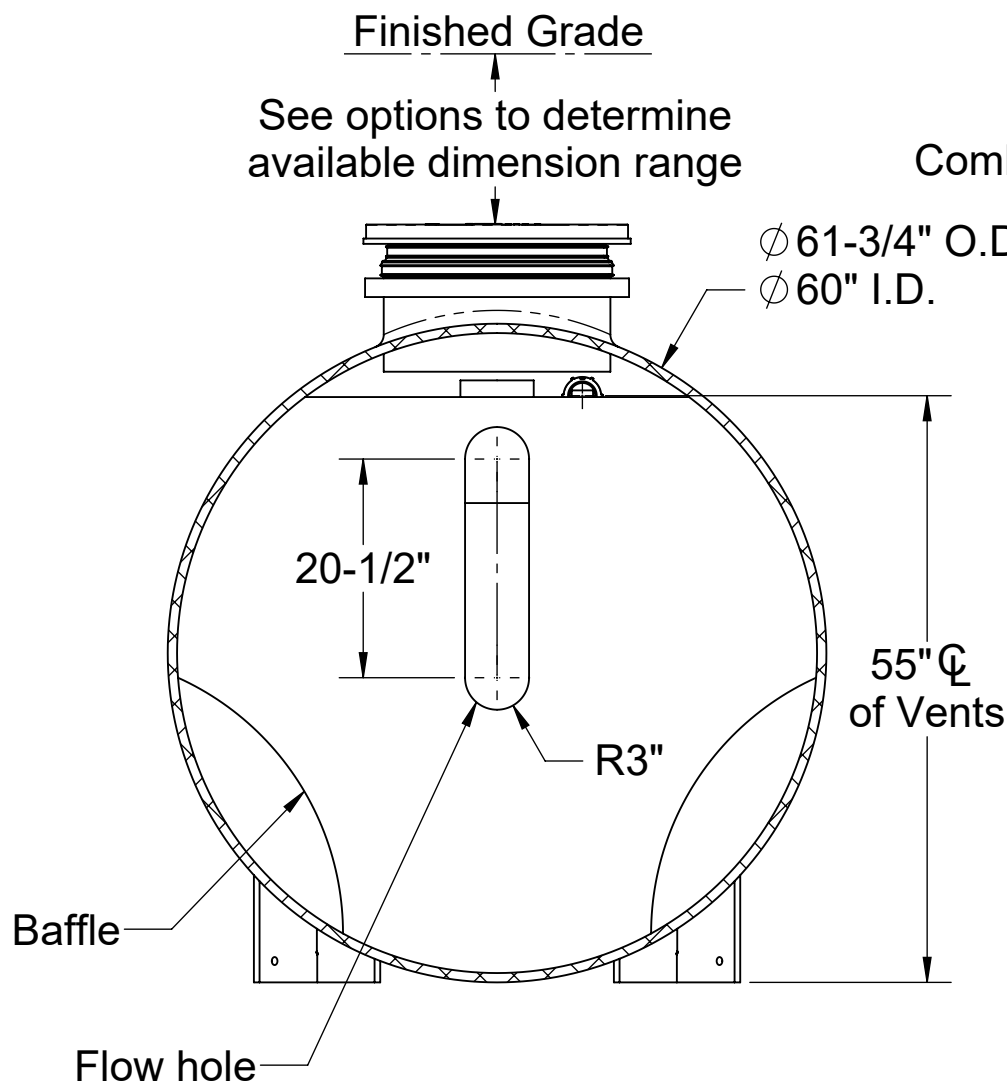
SECTION B-B
