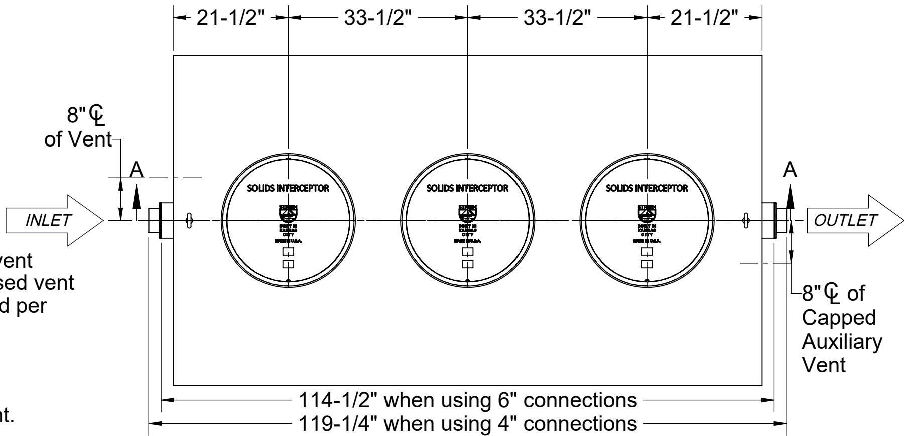
TOP VIEW
