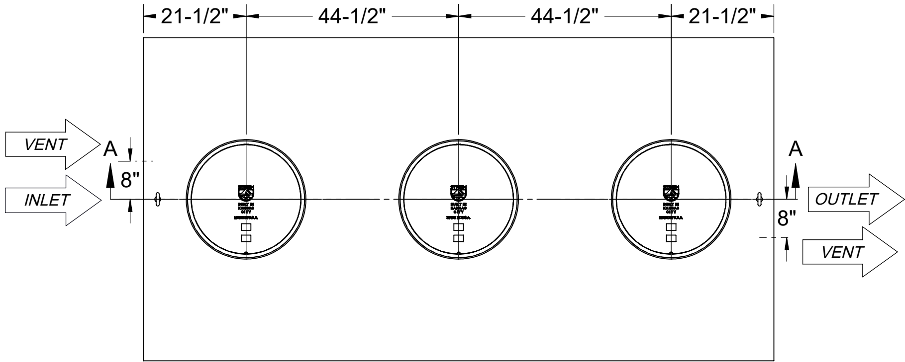
TOP VIEW
