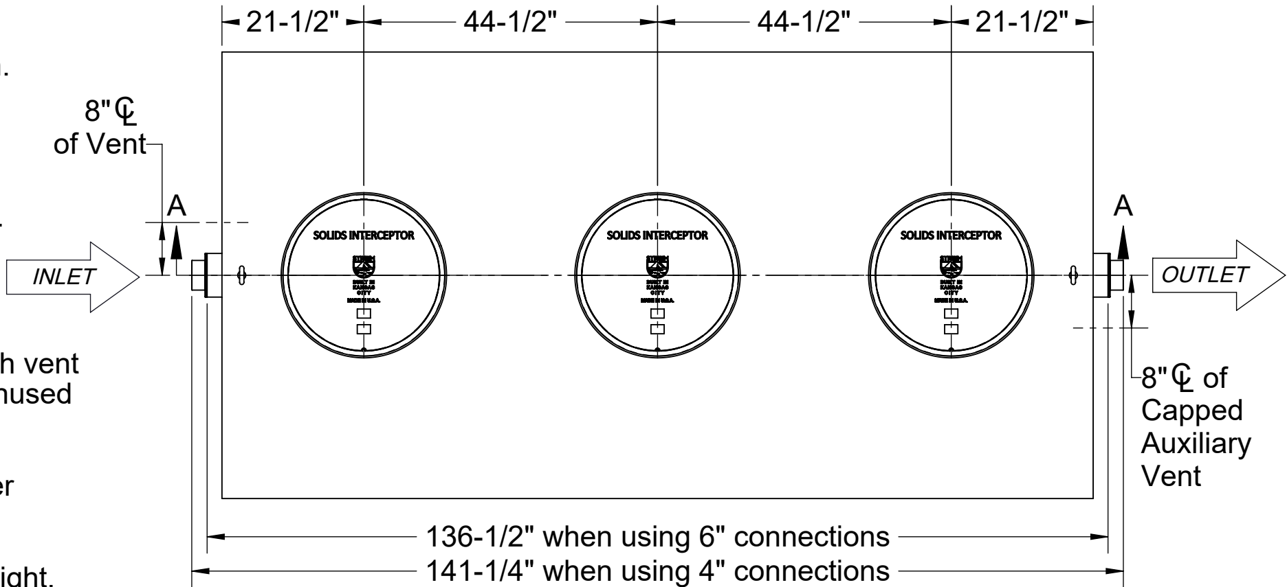
TOP VIEW
