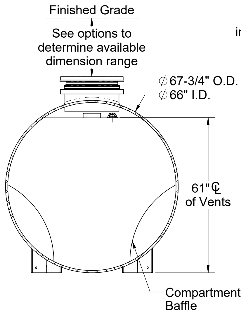
SECTION B-B
