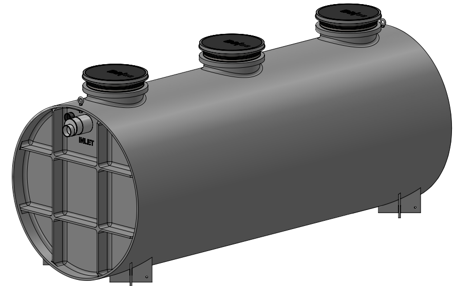
FLI-2000 FLAMMABLE LIQUID INTERCEPTOR 2,000 GAL
