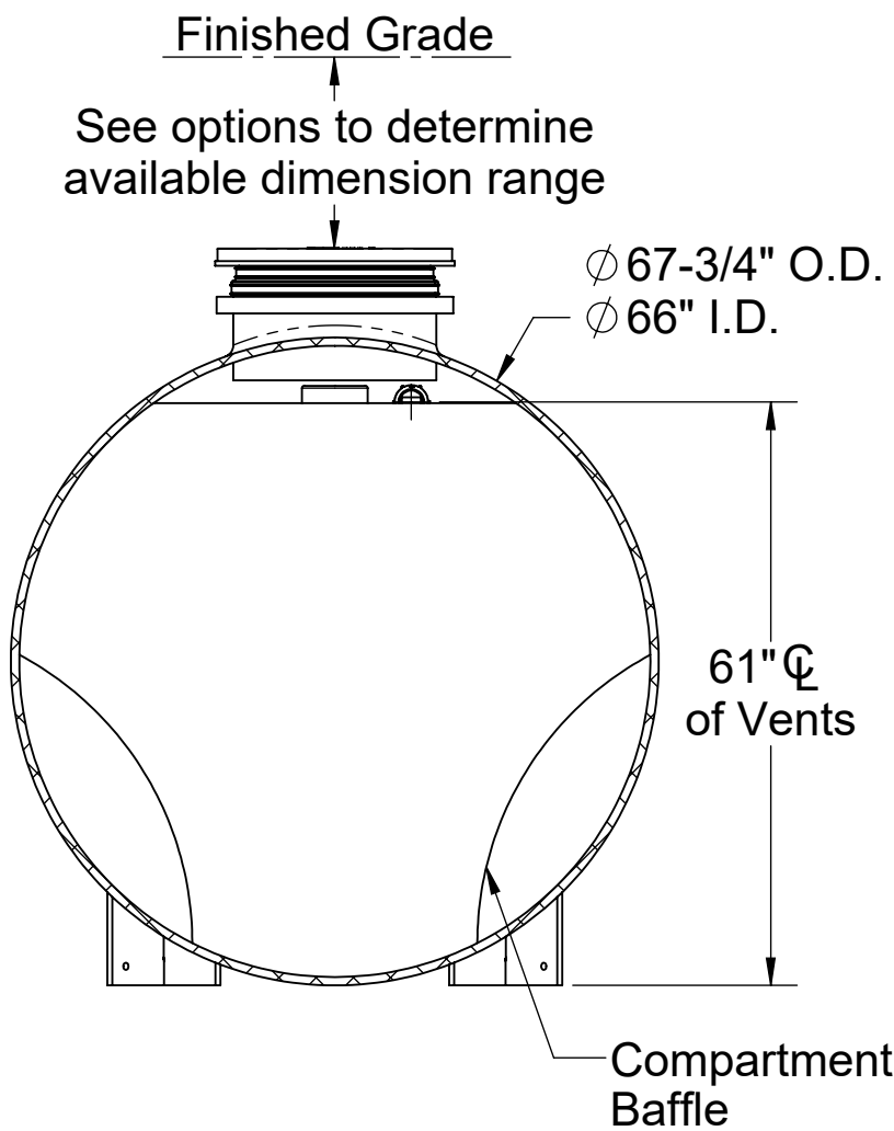
SECTION B-B
