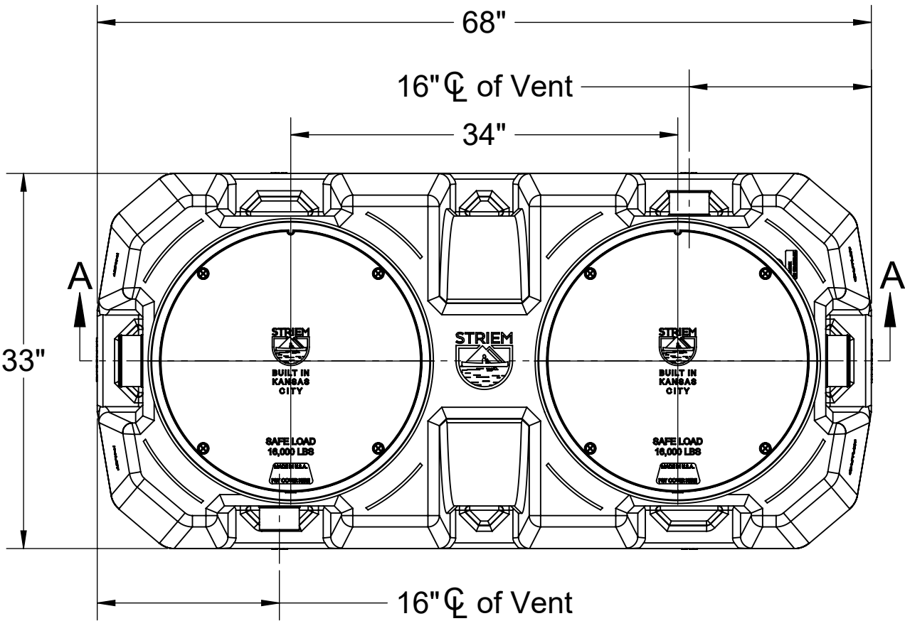
TOP VIEW
