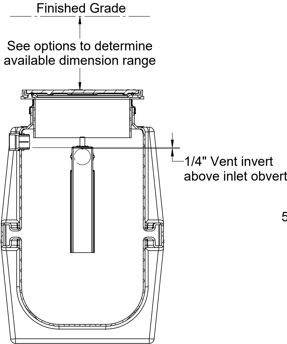
SECTION B-B
