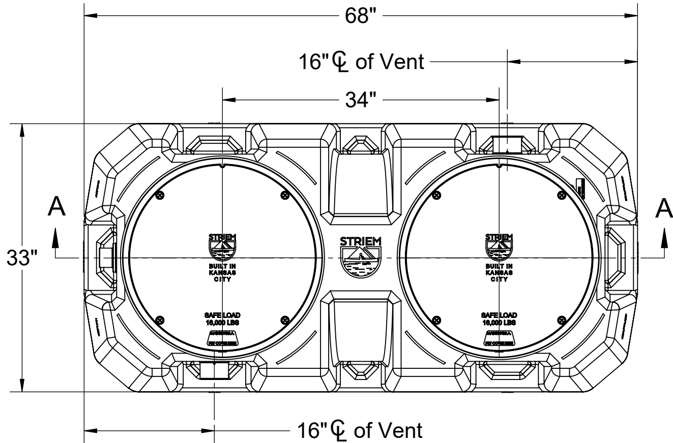
TOP VIEW
