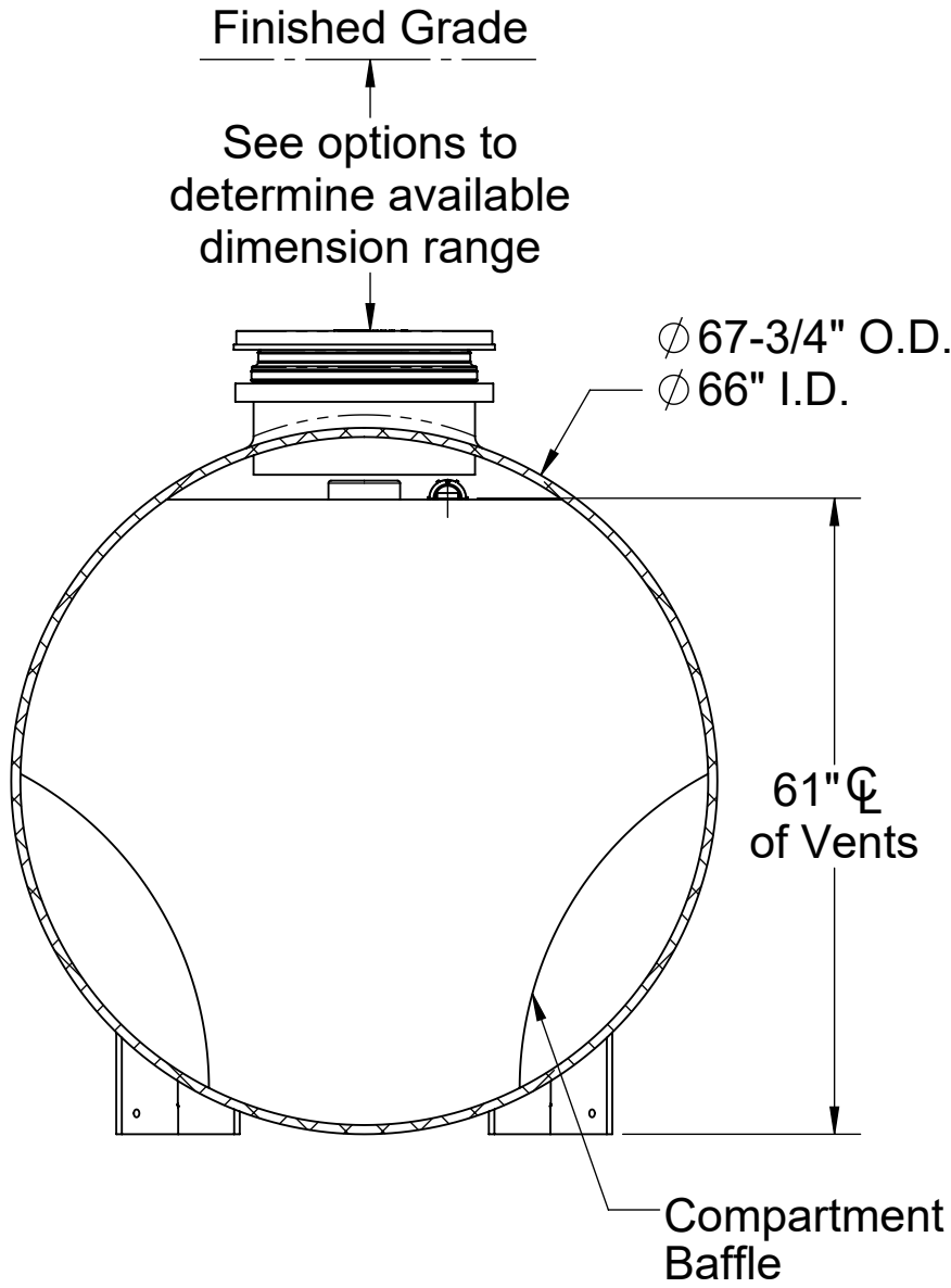
SECTION B-B
