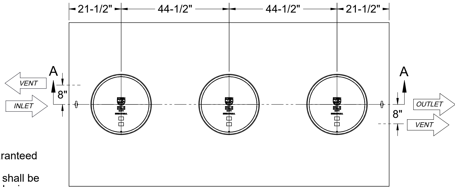
TOP VIEW
