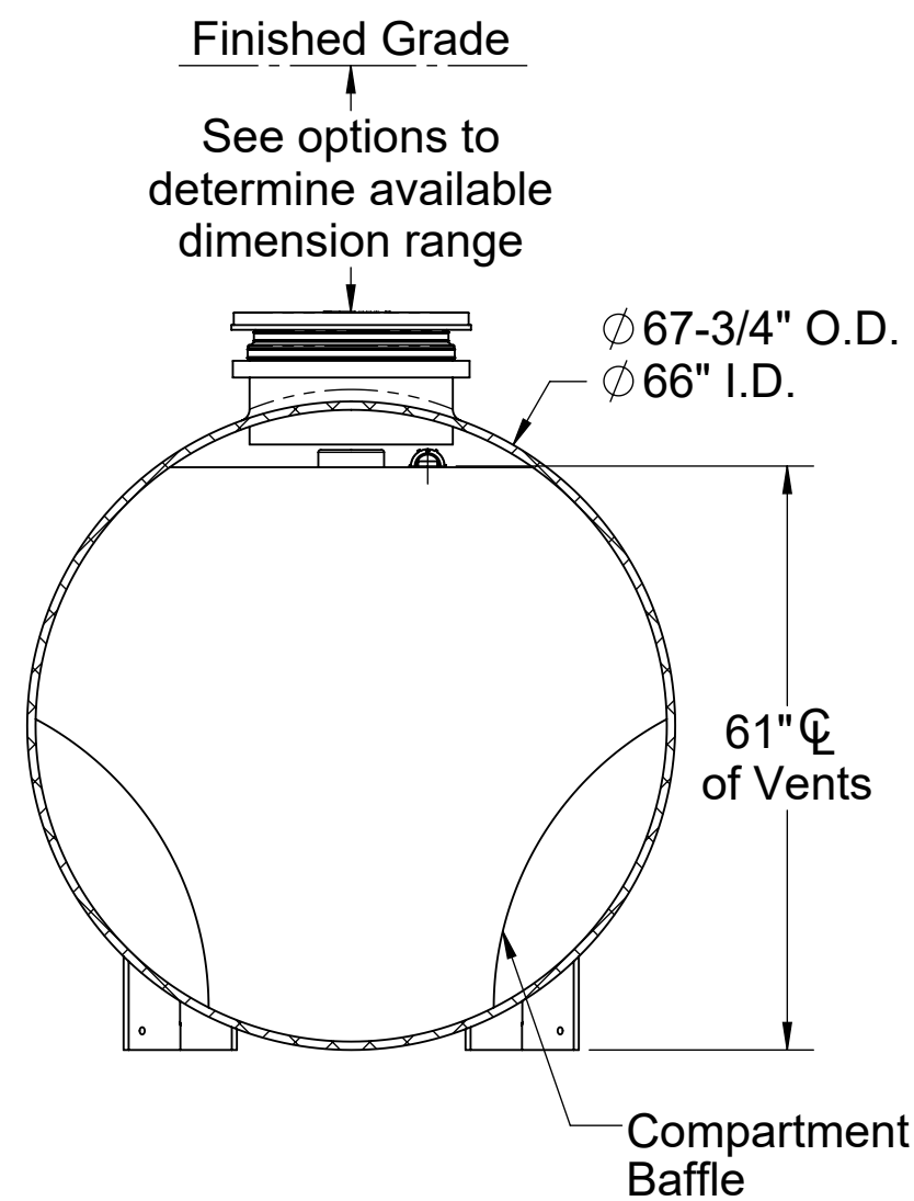
SECTION B-B
