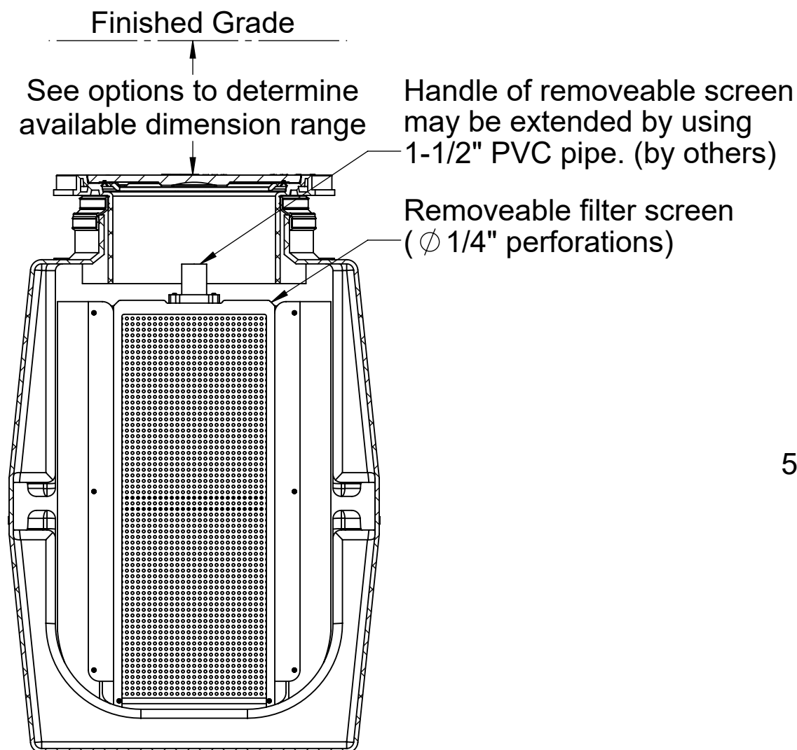
SECTION B-B
