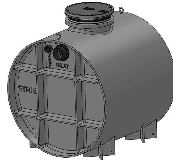
CB-500-S SETTLER SERIES 500 GAL CATCH BASIN
