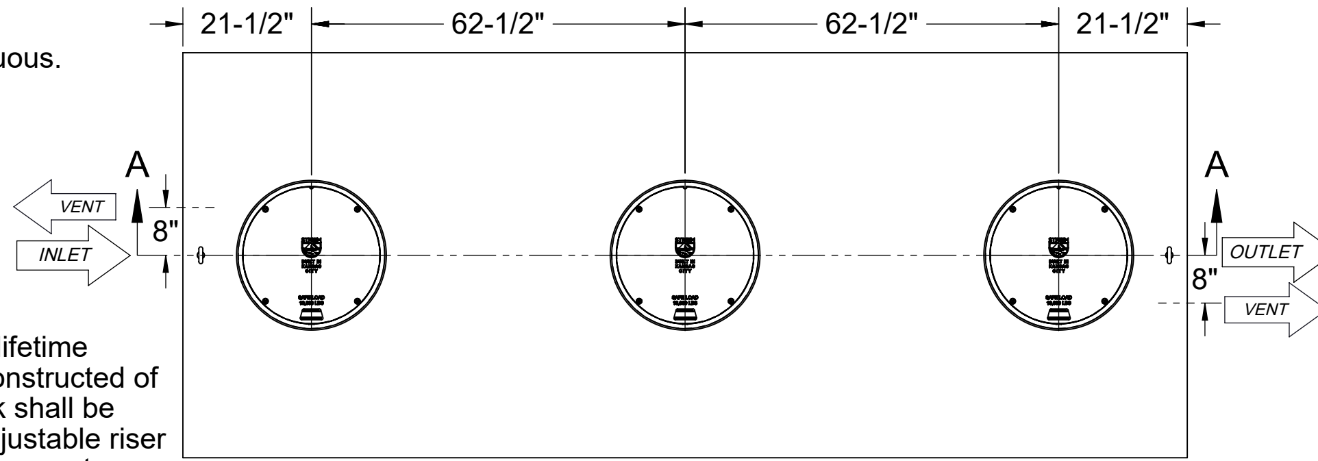
TOP VIEW
