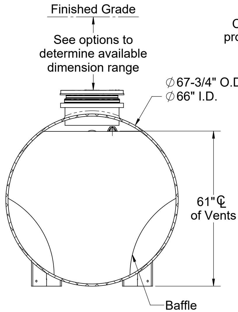
SECTION B-B
