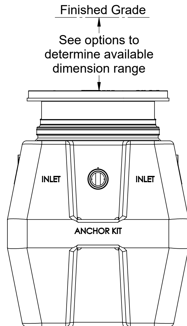
END VIEW
