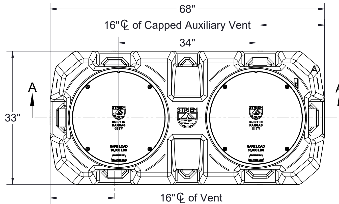
TOP VIEW
