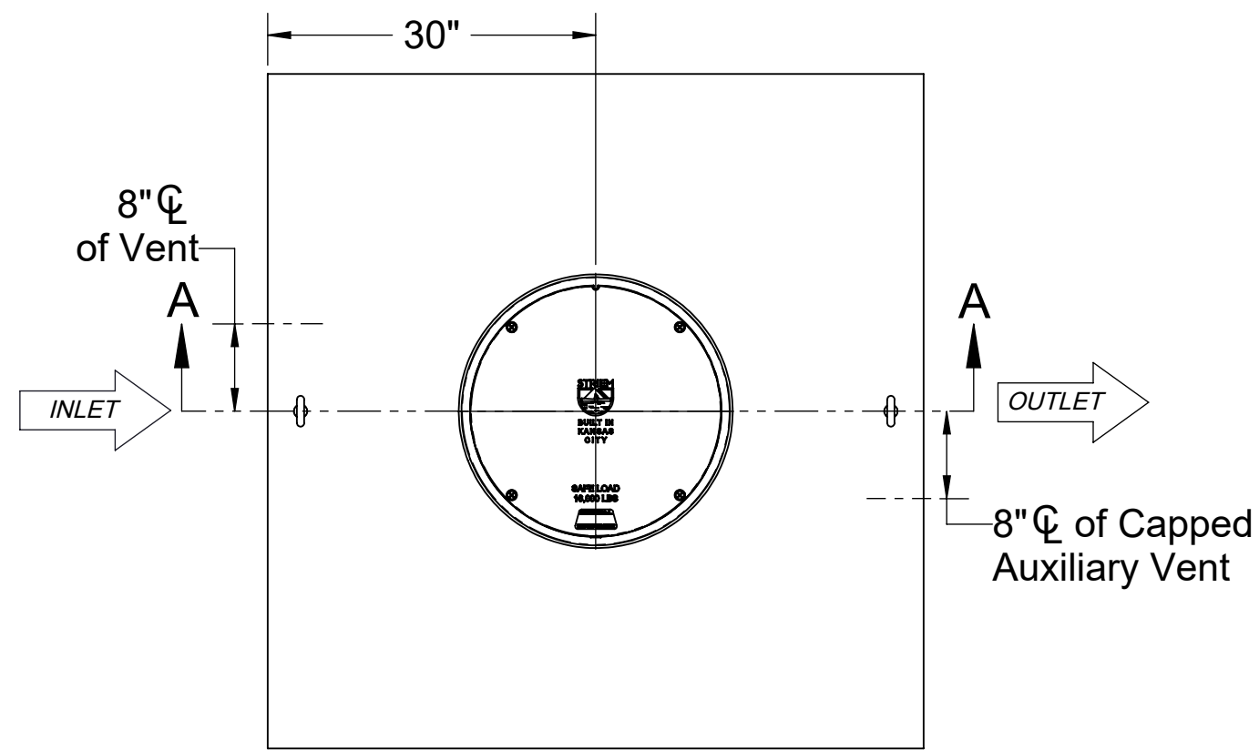
TOP VIEW
