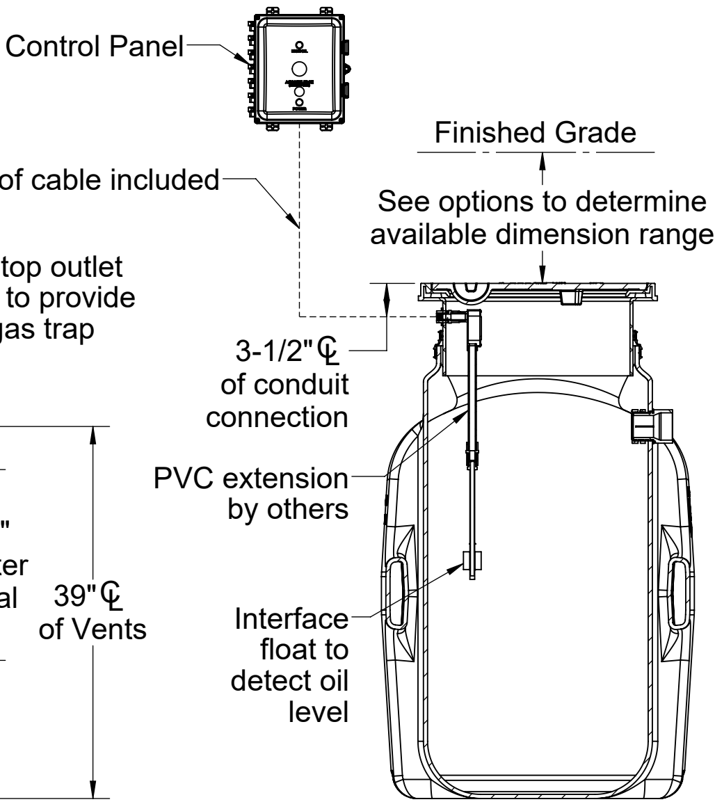
SECTION B-B
