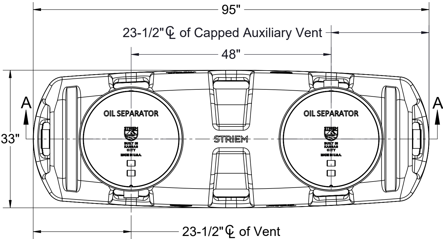
TOP VIEW
