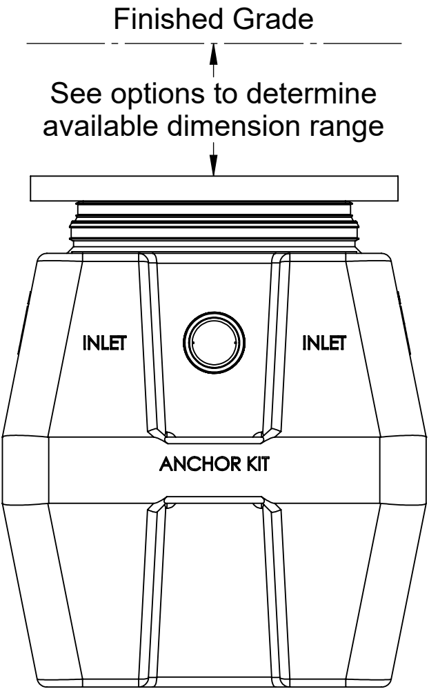
END VIEW
