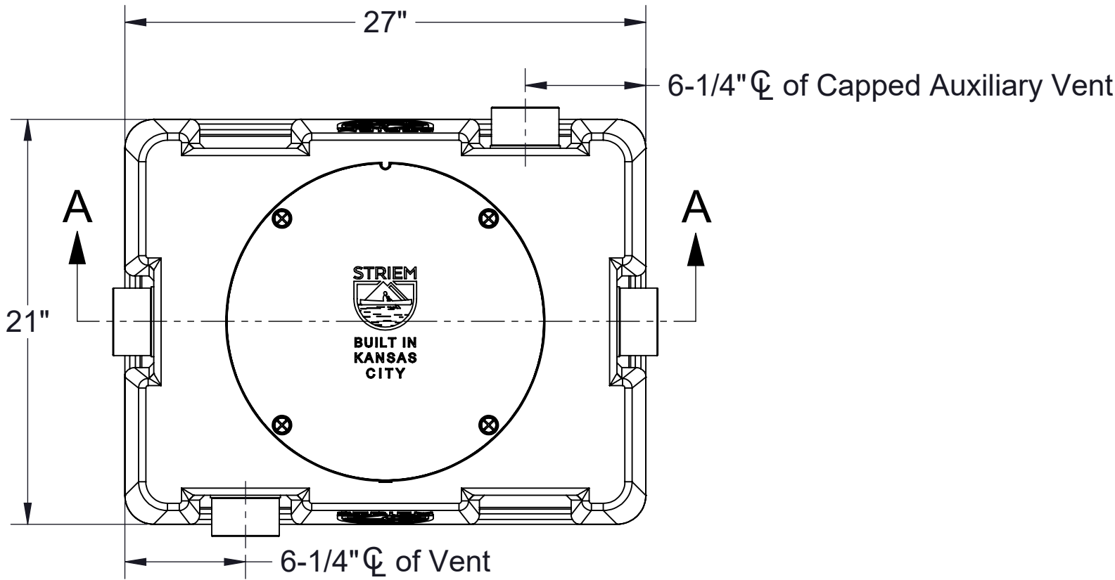
TOP VIEW
